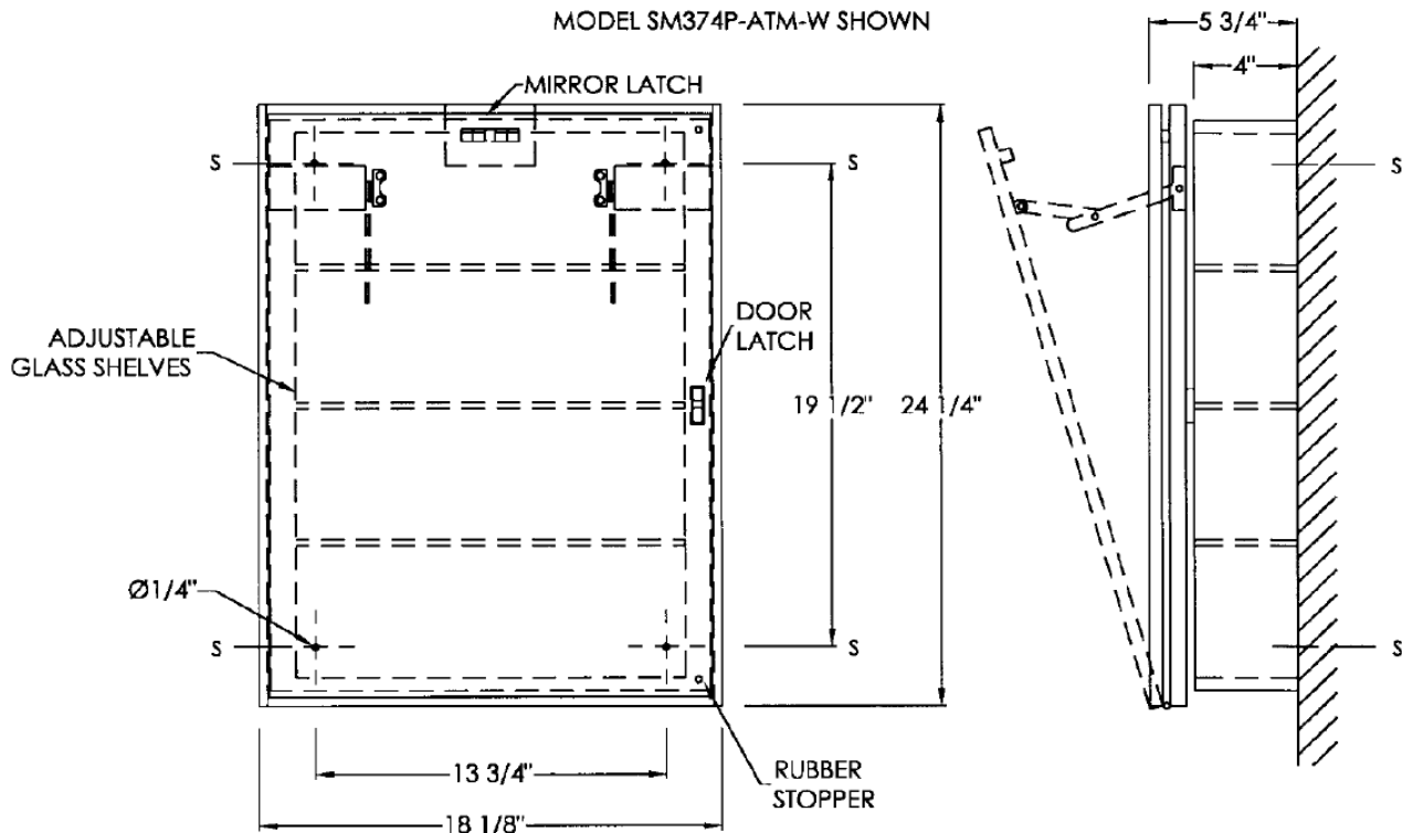
MODEL SM374P-ATM-W SHOWN
