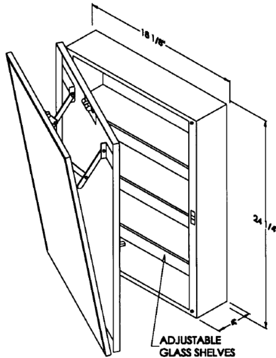
MODEL SM374P-ATM-W SHOWN WITH CABINET OPEN AND MIRROR TILTED
